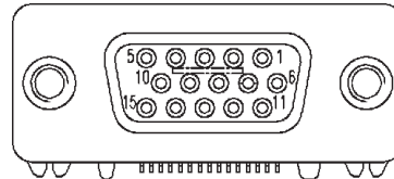
15 Position VESA Receptacle HD-22 Part Number 1734341-1
