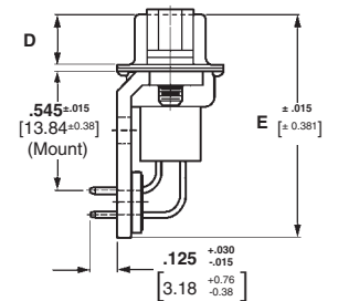
With 4-40 Female Screwlocks
