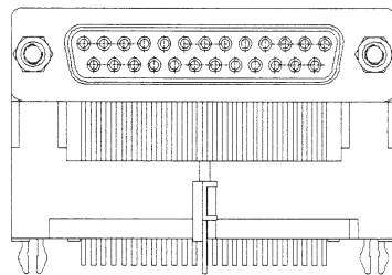
High-Rise 25 Position HD-20 Receptacle
