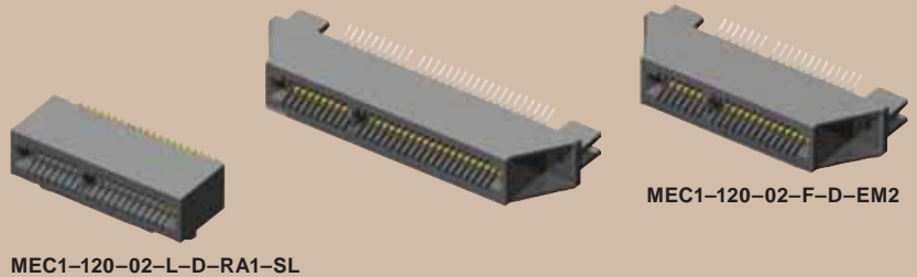
MEC1-120-02-L-D-RA1-SL
