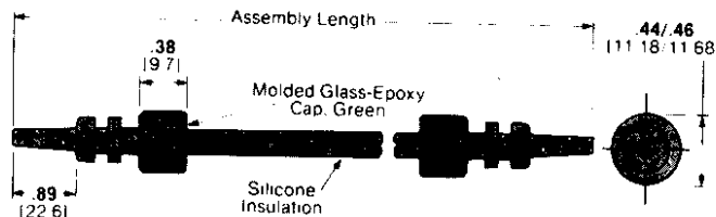
Part Number 830612
