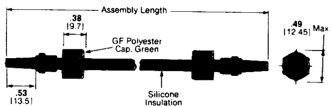
Part Number 862546
