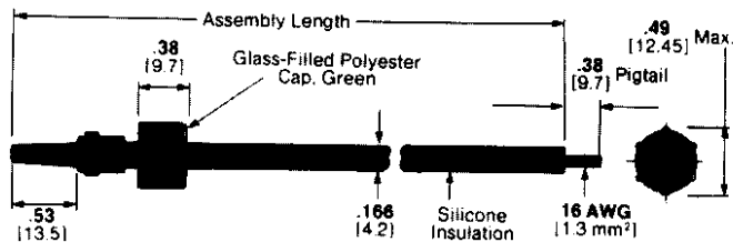
Part Number 862545
