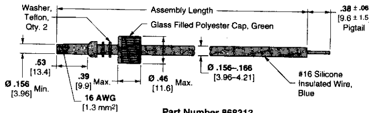
Part Number 868313
