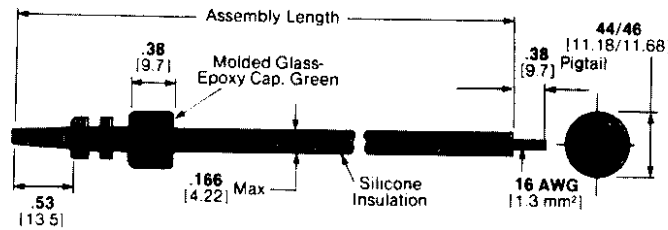
Part Number 830611
