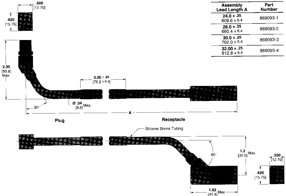
Part Number 869093
