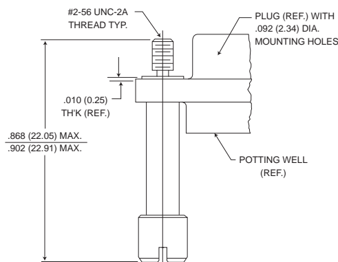
Figure 2. Jackscrew - High Profile Slotted Head Size 9-51 Size 100*
