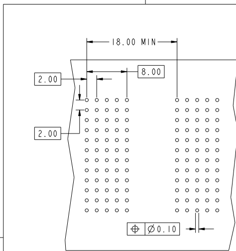
REQUIRED PCB LAYOUT COMPONENT SIDE SEE PRINT 58351 FOR ADDITIONAL PCB INFORMATION
