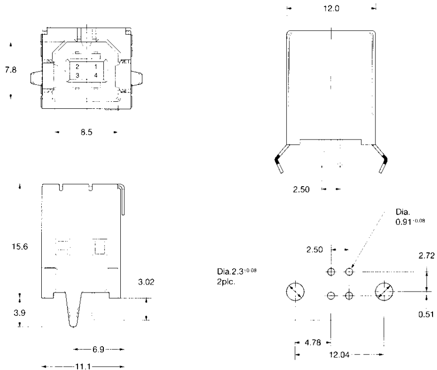
PC Board Layout
