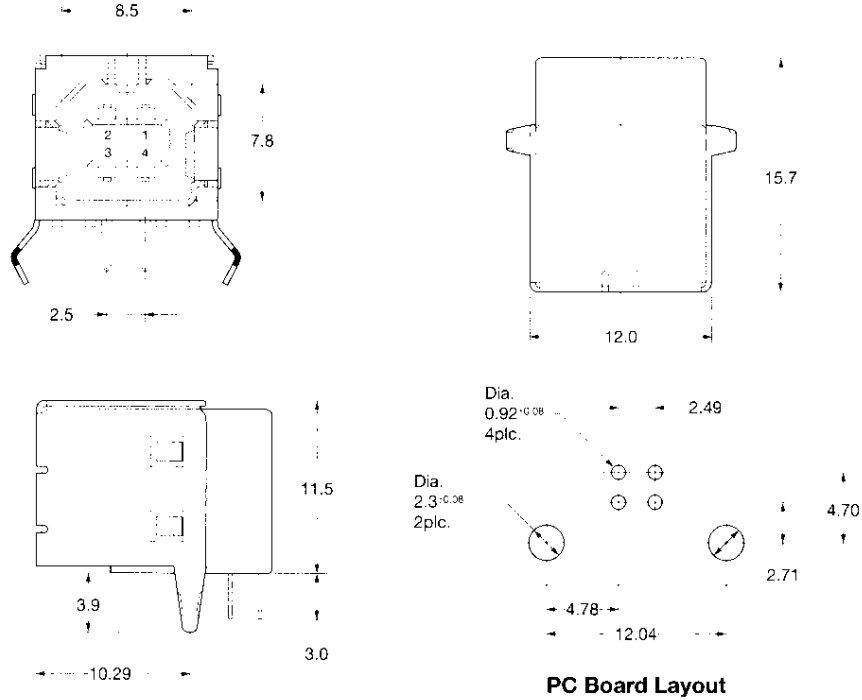
PC Board Layout
