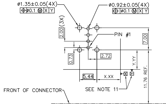
PC BOARD MOUNTING DIMENSIONS FOR 4 PIN
