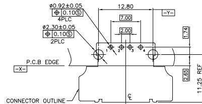
RECOMMENDED P.C.B LAYOUT TOP VIEW, TOLERANCE: ±0.05
