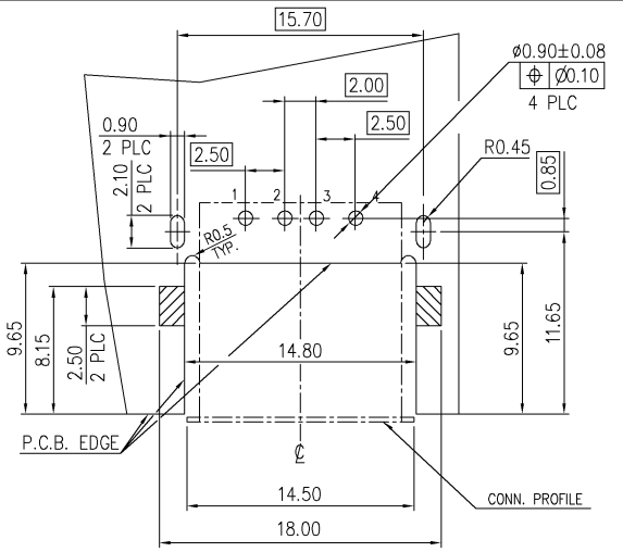
RECOMMEND P.C.B LAYOUT (THICKNESS=1.2mm) (COMPONENT SIDE) TOLERANCE±0.05
