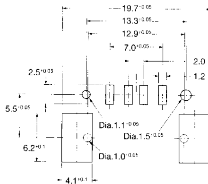
PC Board Layout (Component Side)
