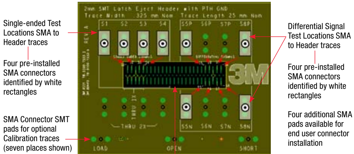
Latch/Eject Header SMT Pads (2x25 places shown) Note: Header will be pre-installed
