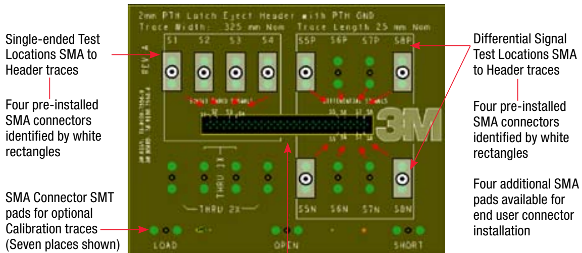
Latch/Eject Header PTH (2x25 places shown) Note: Header will be pre-installed
