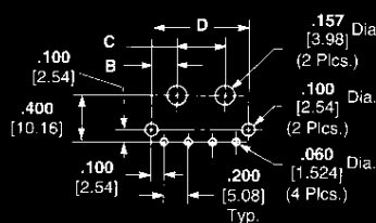
Recommended PC Board Hole Layout .062 [1.57] thick PC Board
