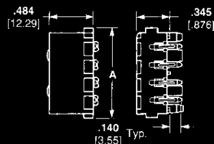
Part Number 770829-1
