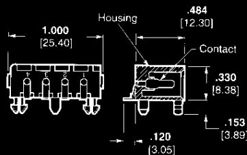
Part Number 770829-1
