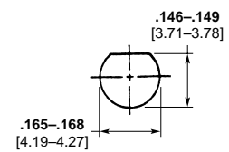
"D" Hole Dimensions For Panel Mounting
