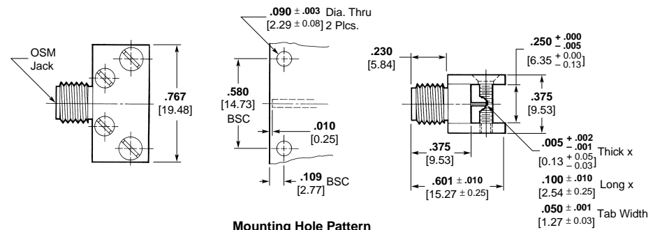
Mounting Hole Pattern
