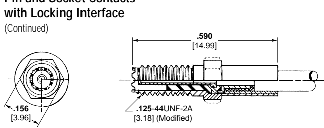
Straight Jack 1 Part Number 141-0017-0001 Instruction Sheet Number 408-08510 Former MICRODOT I.S. Number RF-ASMB-12
