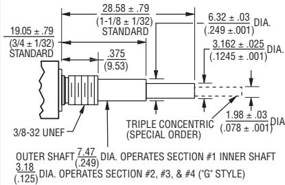
"A" Bushing 3/8 " (9.53 mm) Dia. Plain - Concentric Shaft
