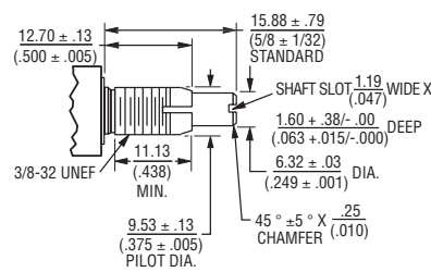
"B" Bushing 3/8 " (9.53 mm) Dia. Plain - Single Shaft
