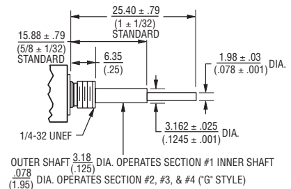
"C" Bushing 1/4 " (6.35 mm) Dia. Plain - Concentric Shaft
