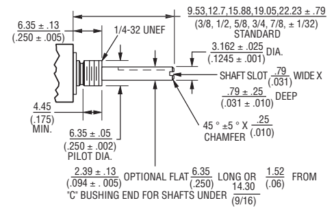
"C" Bushing 1/4 " (6.35 mm) Dia. Plain - Single Shaft
