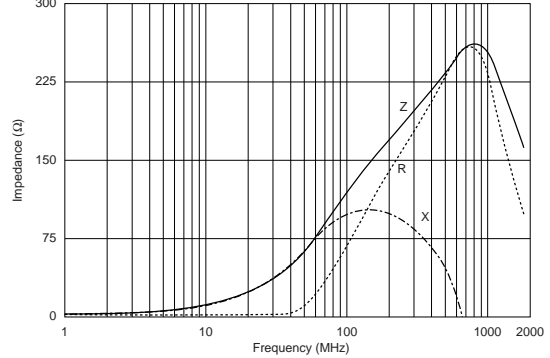
BLM15BD121SN1
