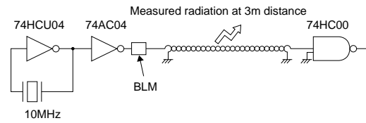
Testing Circuit
