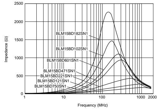
BLM15BD Series
