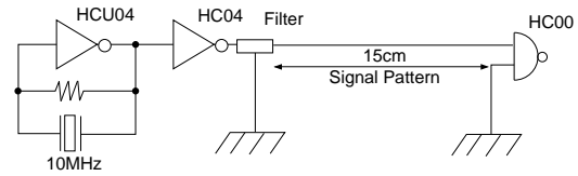
Testing Circuit
