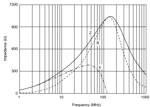
BLA31AG102SN4
