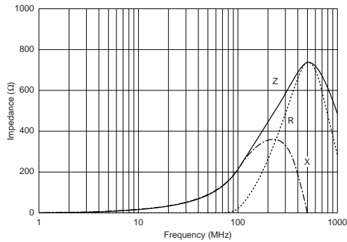
BLA2ABB221SN4
