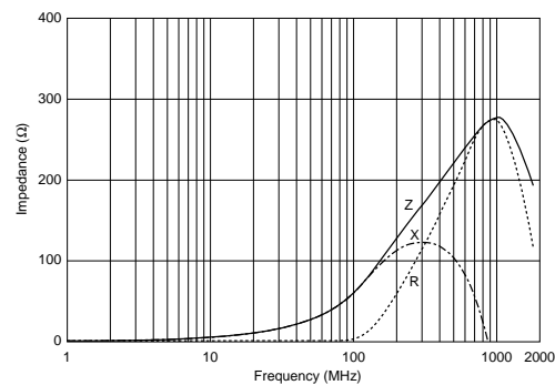
BLM15BB750SN1
