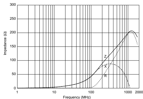
BLM15BB470SN1
