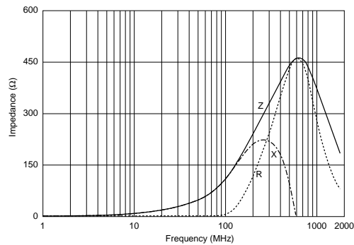
BLM15BB121SN1
