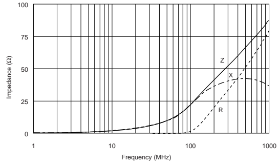
BLA2ABB220SN4
