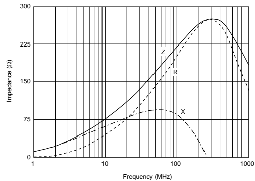
BLA31AG221SN4
