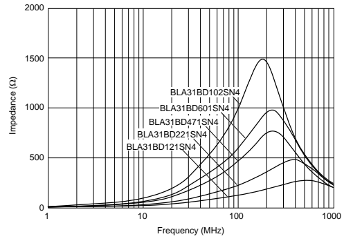
BLA31B Series
