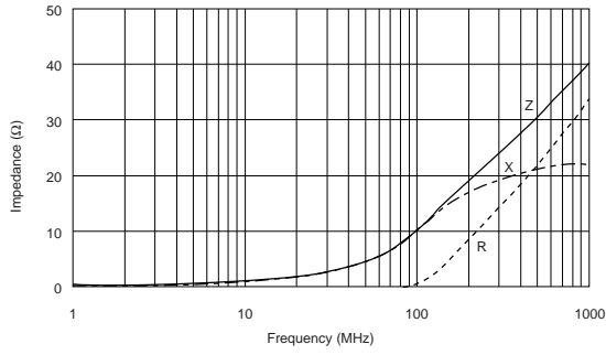
BLA2ABB100SN4
