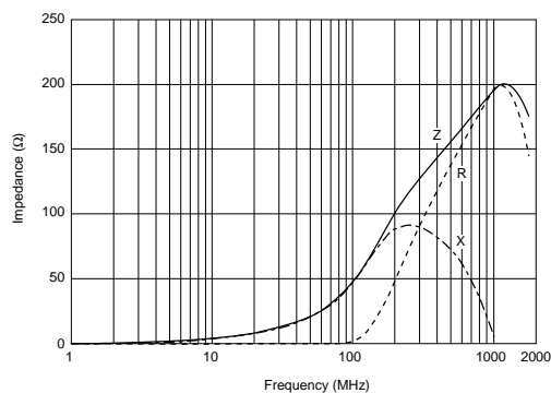
BLM18BB470SN1
