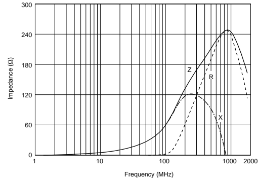
BLM18BB600SN1
