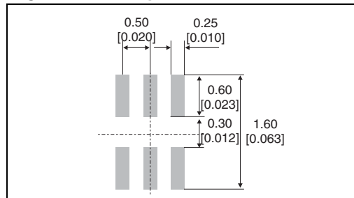
Figure 8. Footprint in mm [inches]
