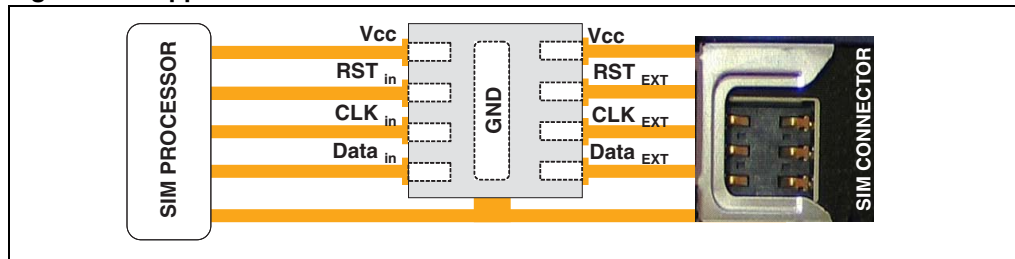
Figure 11. Application schematic
