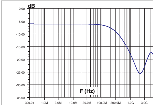
Figure 5. S21(db) attenuation (DATA line)
