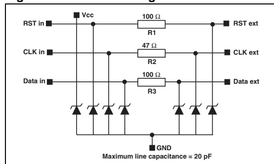
Figure 2. Device configuration
