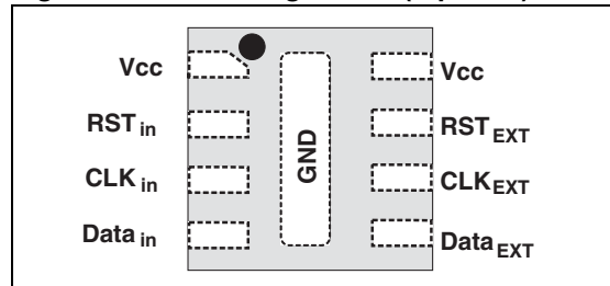
Figure 1. Pin configuration (top view)
