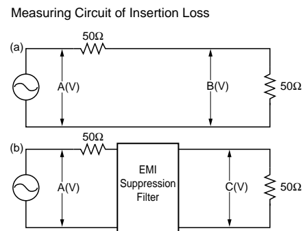
Measuring Circuit of Insertion Loss
