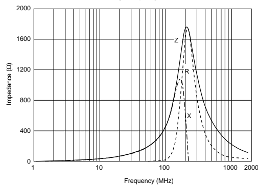
BLM18BB471SN1
