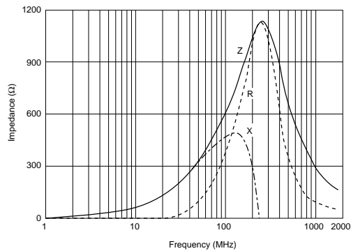
BLM18BD601SN1
