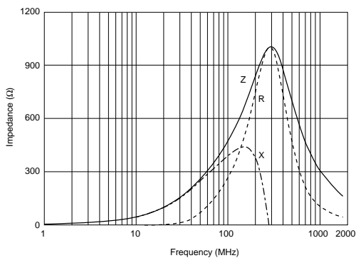
BLM18BD471SN1
