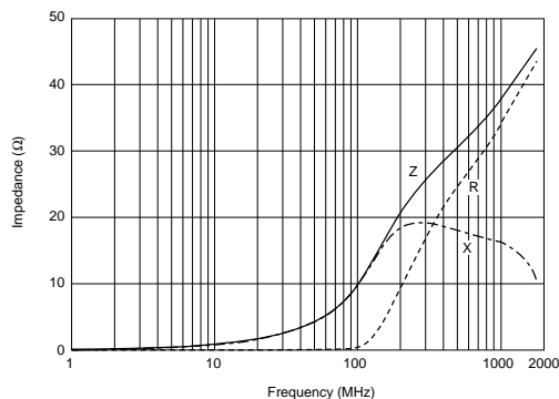
BLM18BB100SN1
