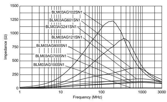
BLM03A Series
