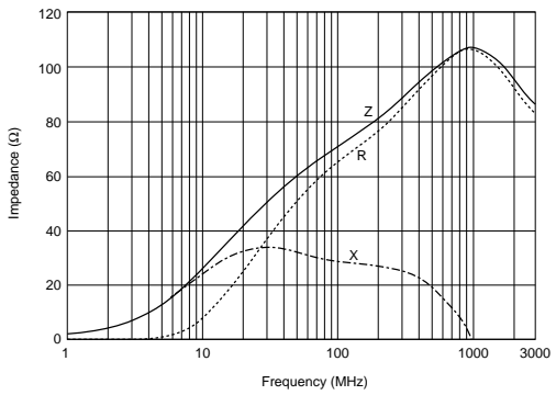
BLM03AG700SN1
