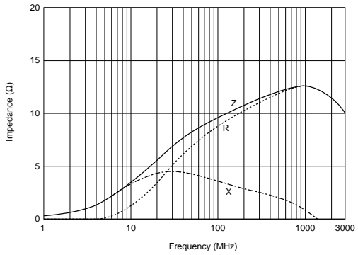
BLM03AG100SN1
