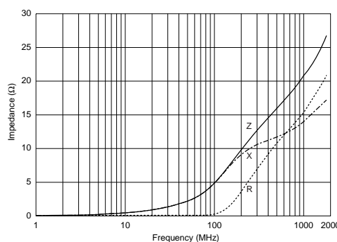
BLM15BB050SN1
