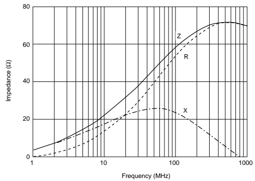
BLA31AG600SN4
