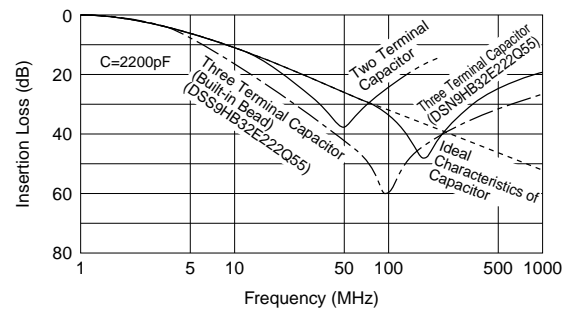
Comparison of Insertion Loss Characteristics
