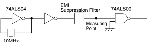
Measuring Circuit
