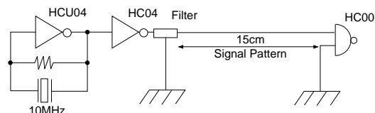
Testing Circuit
