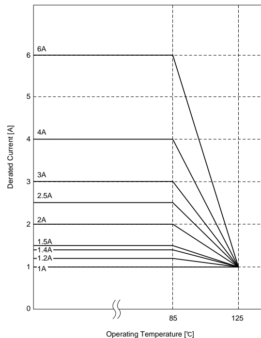
Derating
