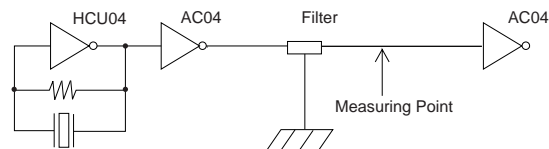
Testing Circuit
