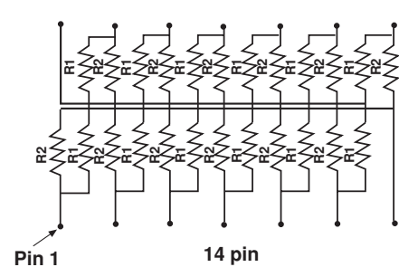
05 Circuit
