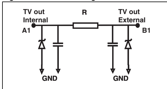
Figure 2. Device configuration
