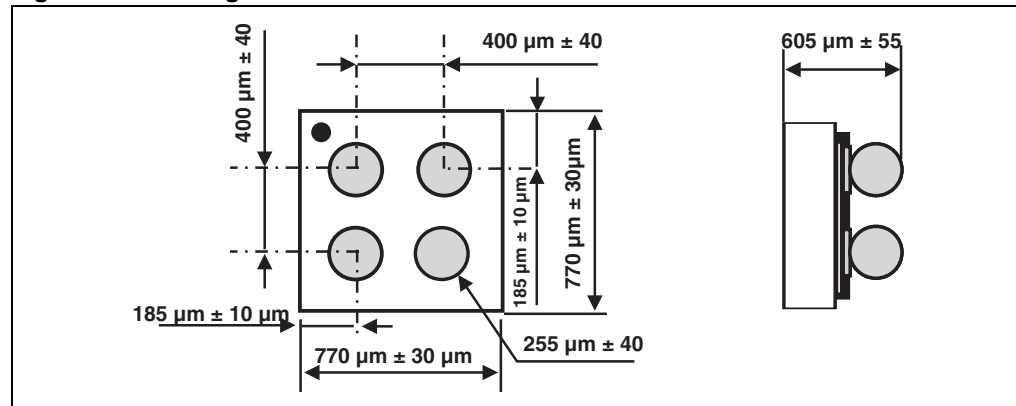
Figure 10. Package dimensions
