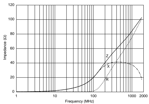
BLM15BB220SN1
