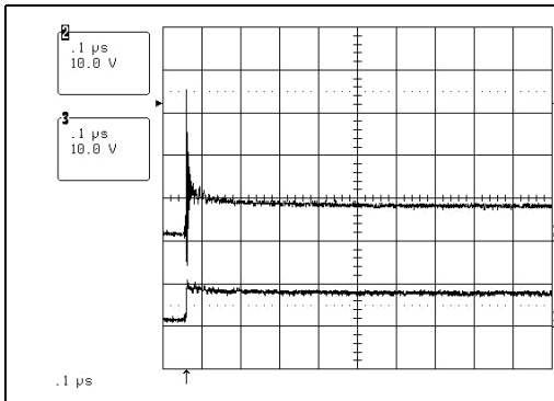
Figure 5. ESD response to IEC 61000-4-2 (+15kV contact discharge)
