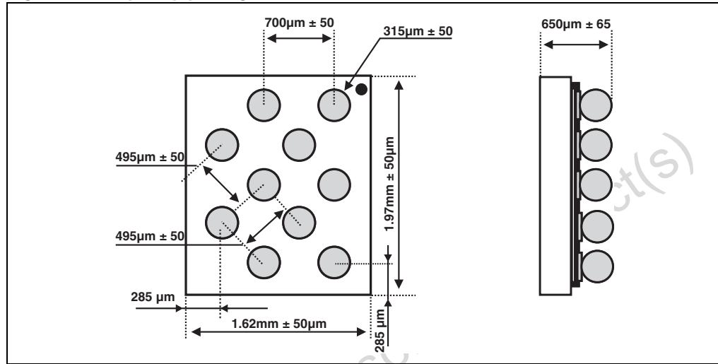
Figure 11. Footprint recommendations Figure 12. Marking
