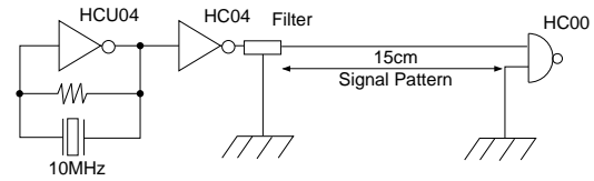
Testing Circuit
