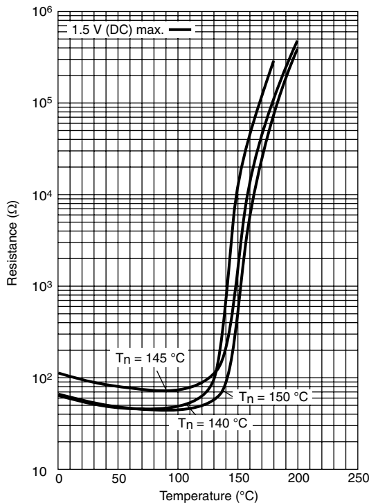
TYPICAL RESISTANCE/TEMPERATURE CHARACTERISTIC FOR 2381 671 91..2, 91083 and 91..4
