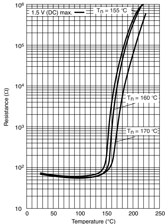
TYPICAL RESISTANCE/TEMPERATURE CHARACTERISTIC FOR 2381 671 91..5, 91..6 and 91..7
