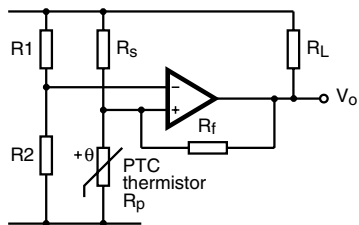
Fig. 1 Typical comparator circuit
