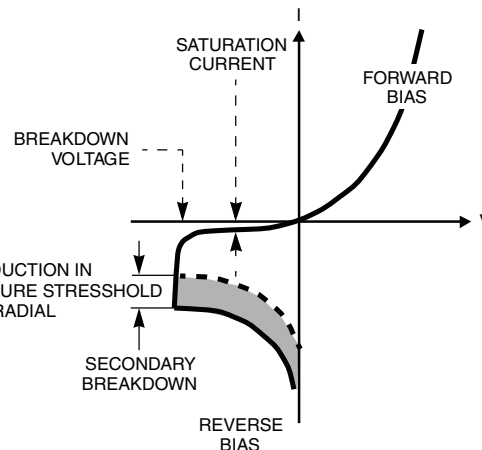
FIGURE 3. V-I CHARACTERISTIC OF PN-JUNCTION
