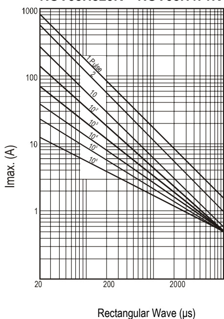
ROV05H820K – ROV05H471K
