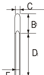
STRAIGHT LEAD TYPE (-S) Table of C max., F, and B_1 max.
