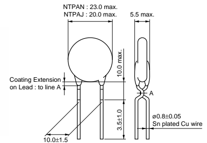
NTPAN/NTPAJ Series
