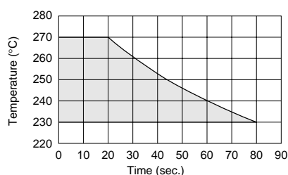
Allowable Reflow Soldering Temperature and Time
