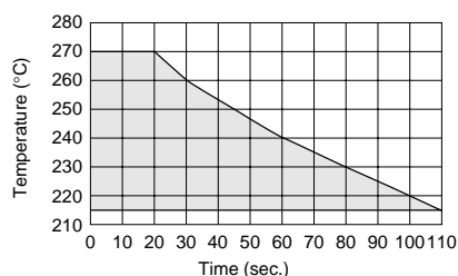
Allowable Reflow Soldering Temperature and Time
