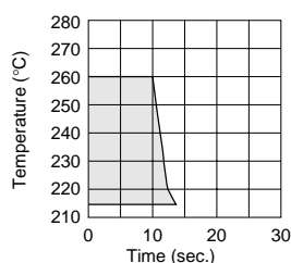
Allowable Flow Soldering Temperature and Time
