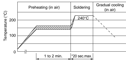
Reflow Soldering Conditions
