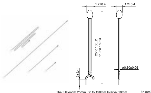
NXFT15_1B Type(twist)
