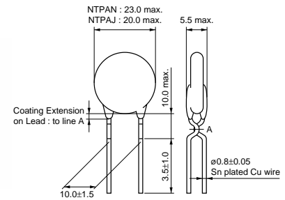
NTPAN/NTPAJ Series
