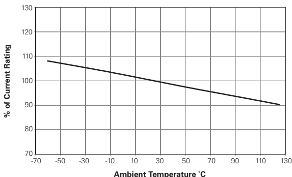
Figure FT1 Thermal Derating Curve (Normalized) for FT600 Devices
