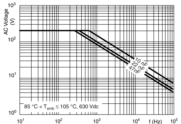
379 - Max. AC voltage as a function of frequency
