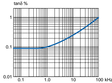
Dissipation factor vs. frequency (at +23°C)
