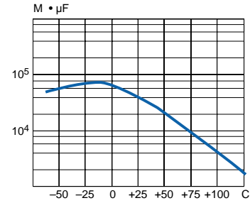
Insulation resistance vs. temperature
