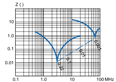
Resonance frequencies CMK 5
