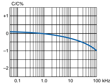
Capacitance vs. frequency (at +23°C)
