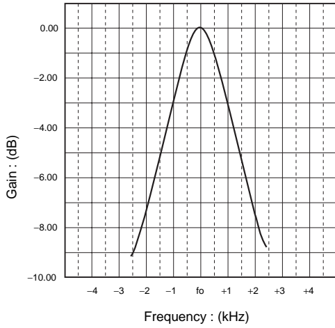
Fig.6 BPF characteristic
