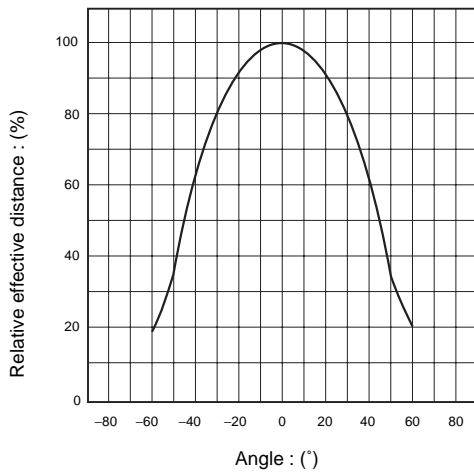
Fig.8 Direction characteristic (Horizontal direction)
