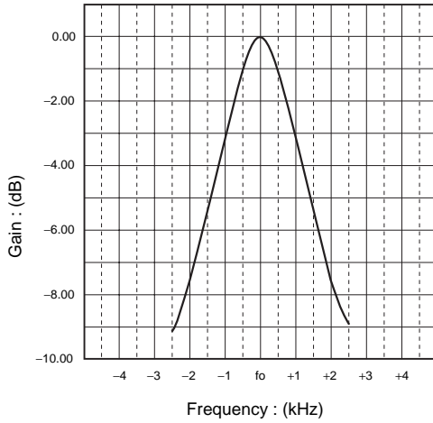
Fig.6 BPF characteristic
