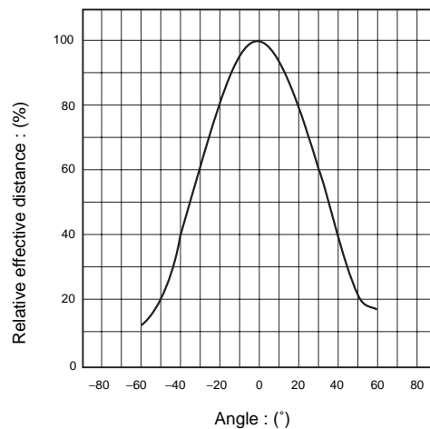
Fig.9 Direction characteristic (Vertical direction)
