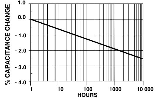
TYPICAL PARAMETER X7R AGING RATE
